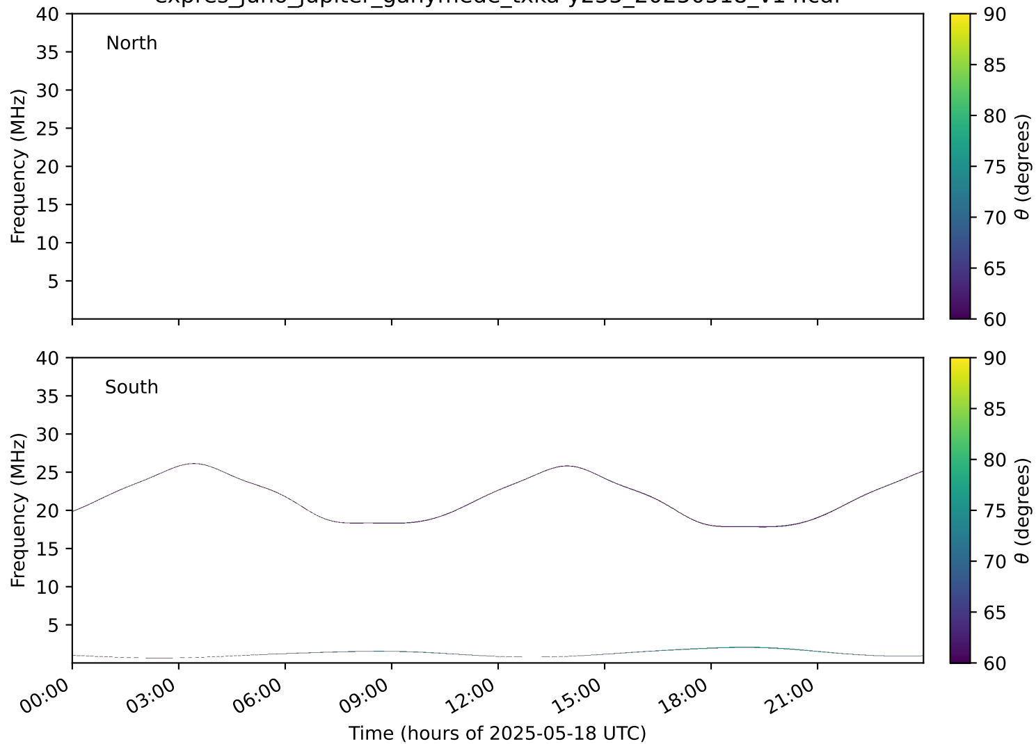
expres_juno_jupiter_ganymede_txka-y235_20250518_v14.cdf
