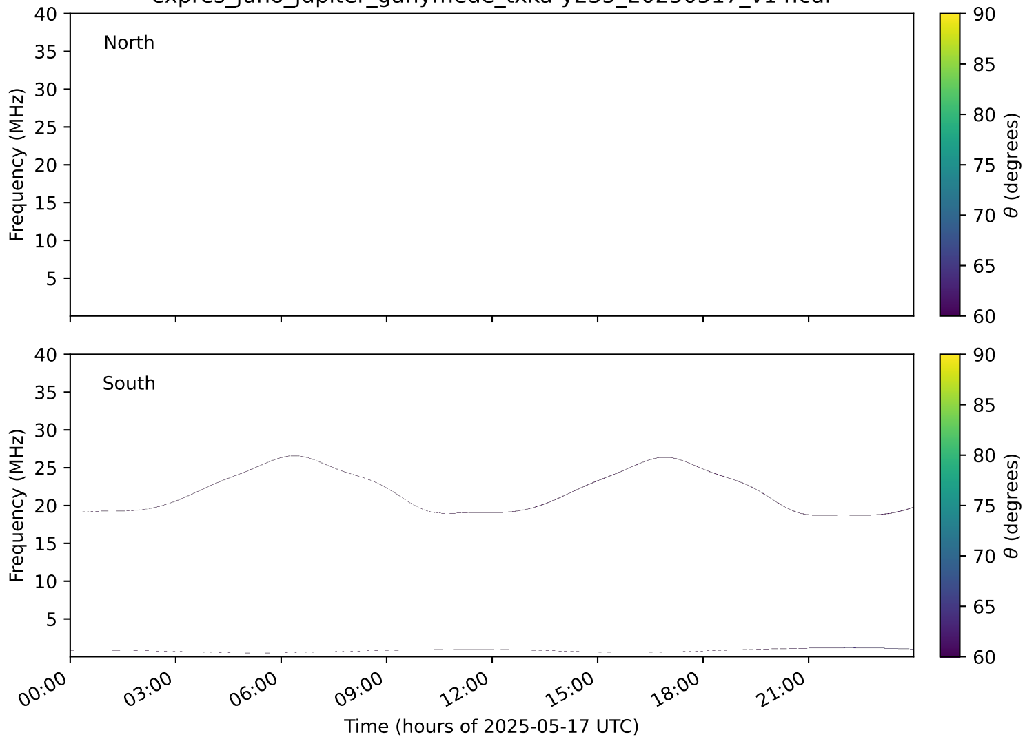
expres_juno_jupiter_ganymede_txka-y235_20250517_v14.cdf
