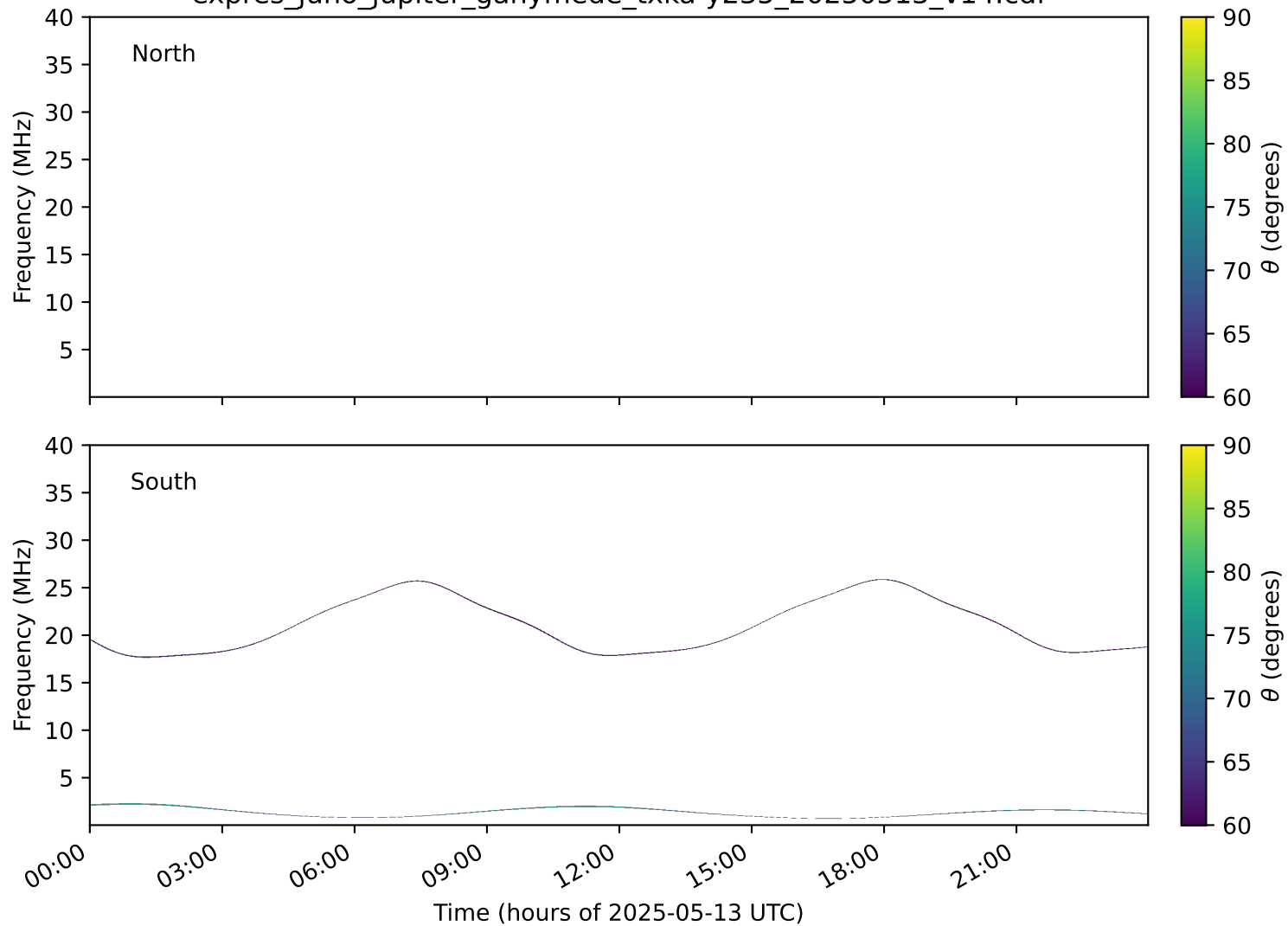
expres_juno_jupiter_ganymede_txka-y235_20250513_v14.cdf
