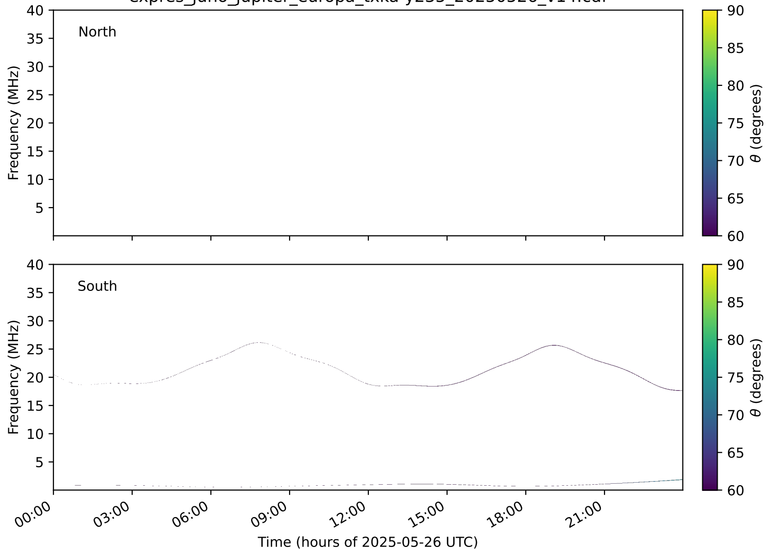
expres_juno_jupiter_europa_txka-y235_20250526_v14.cdf
