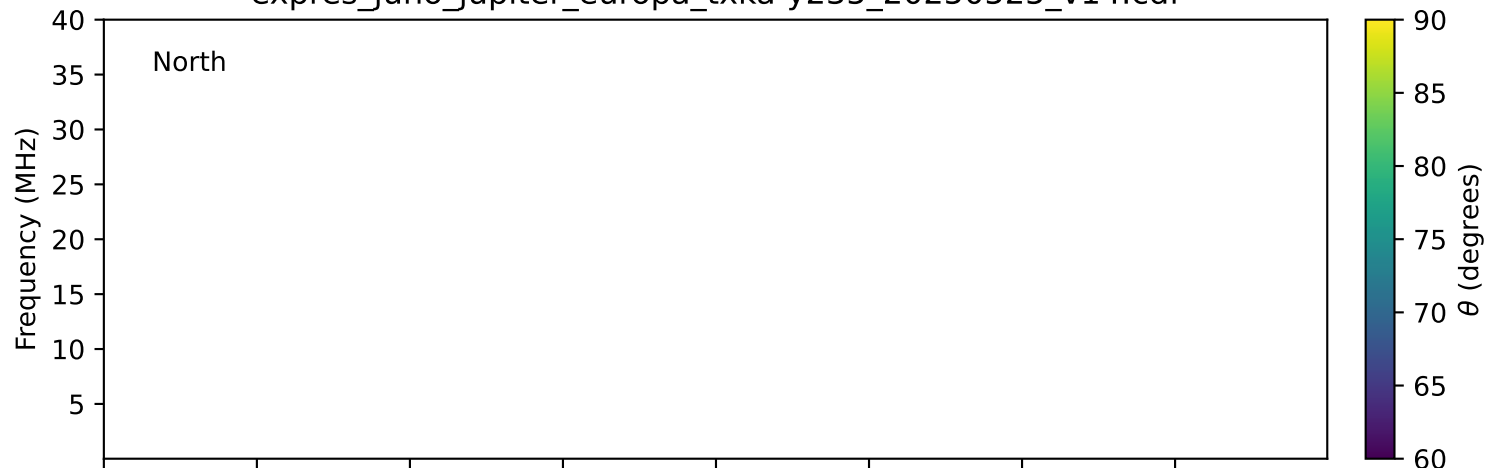
expres_juno_jupiter_europa_txka-y235_20250525_v14.cdf
