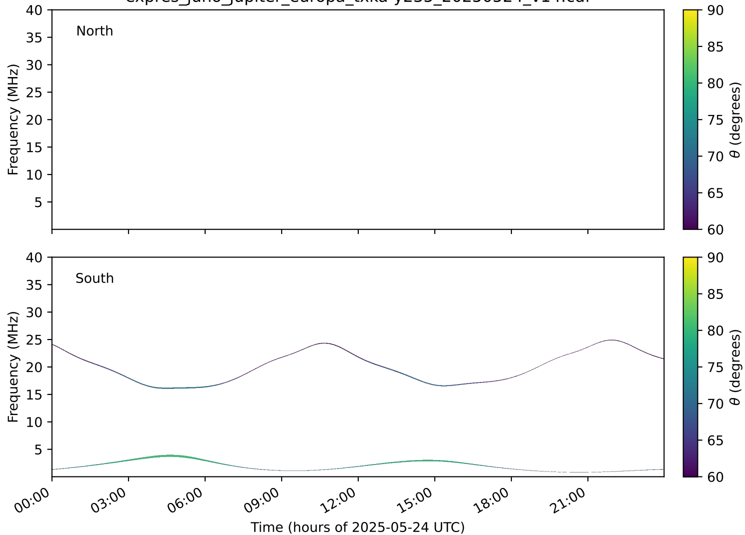
expres_juno_jupiter_europa_txka-y235_20250524_v14.cdf
