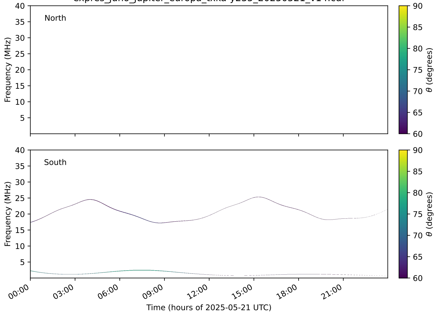
expres_juno_jupiter_europa_txka-y235_20250521_v14.cdf
