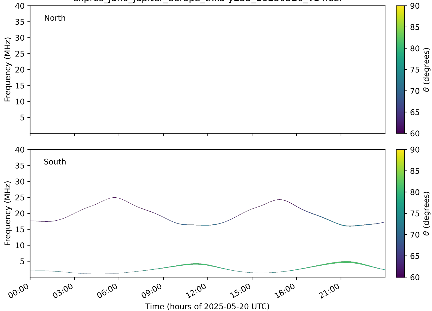
expres_juno_jupiter_europa_txka-y235_20250520_v14.cdf
