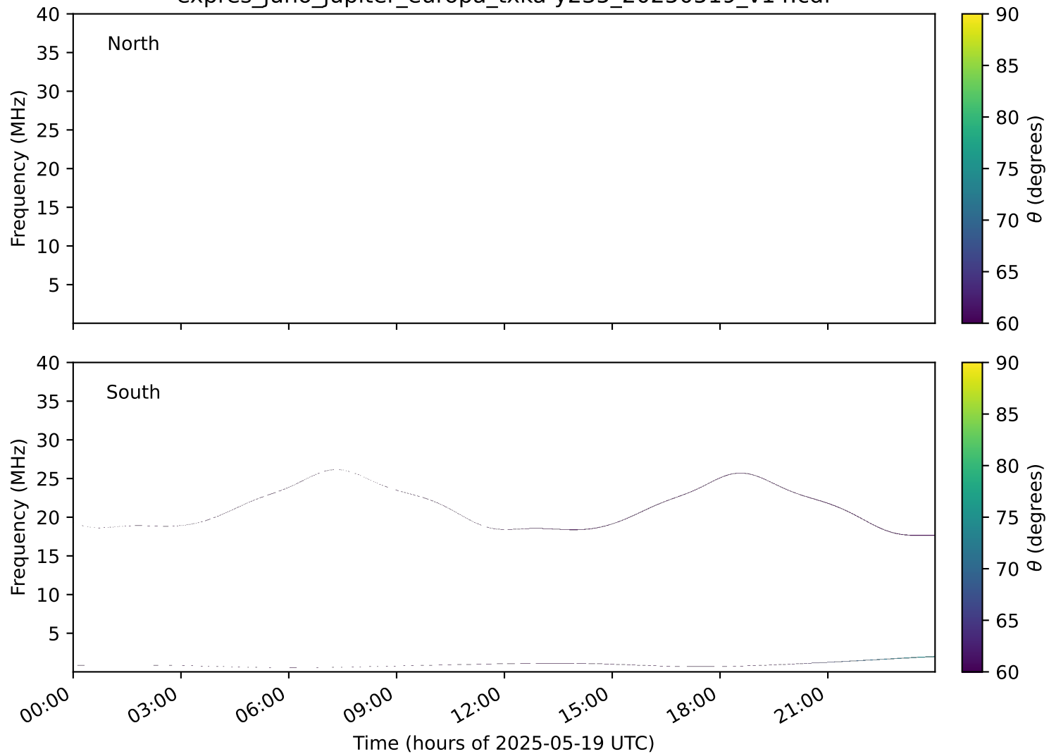
expres_juno_jupiter_europa_txka-y235_20250519_v14.cdf
