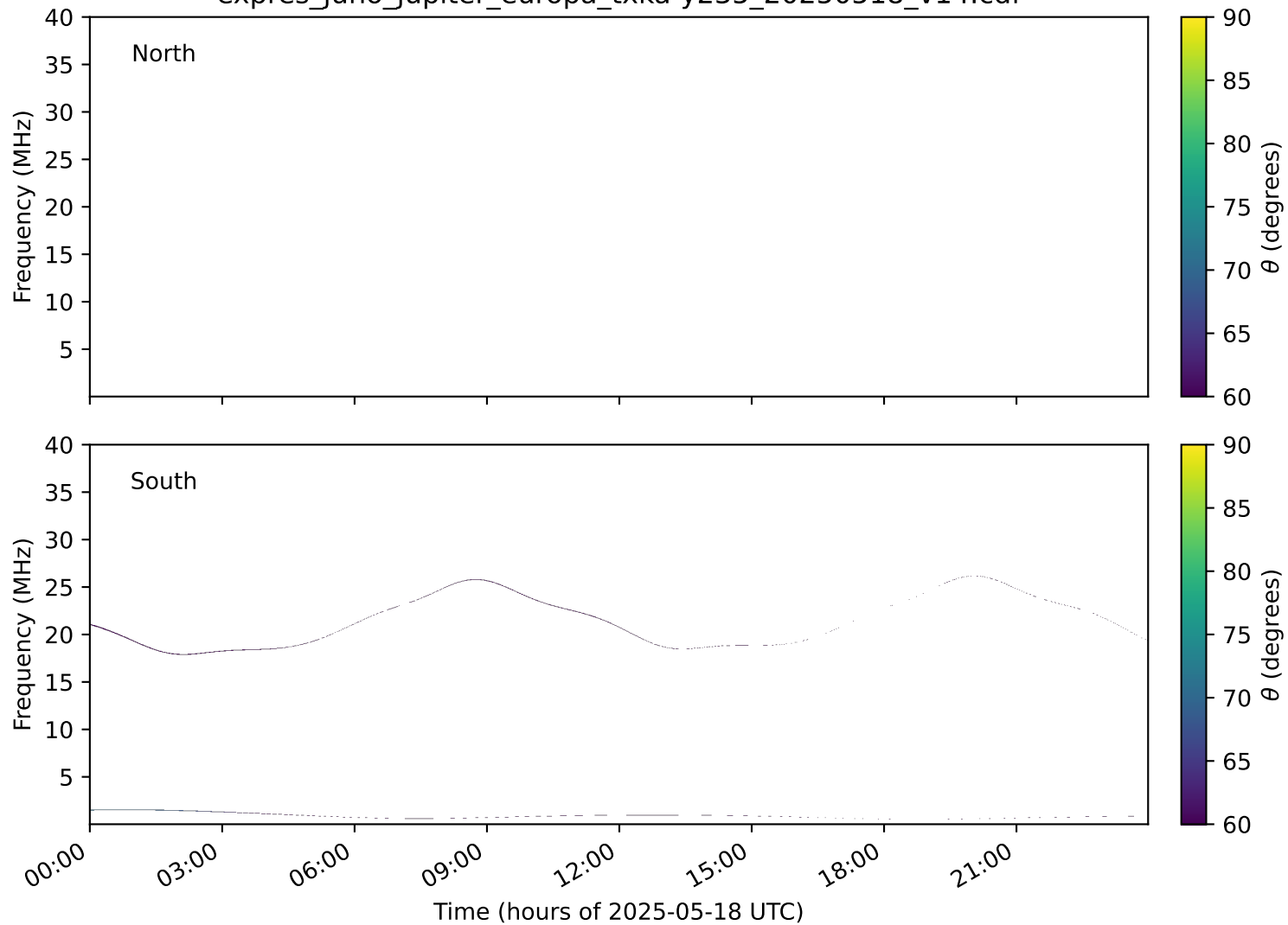
expres_juno_jupiter_europa_txka-y235_20250518_v14.cdf
