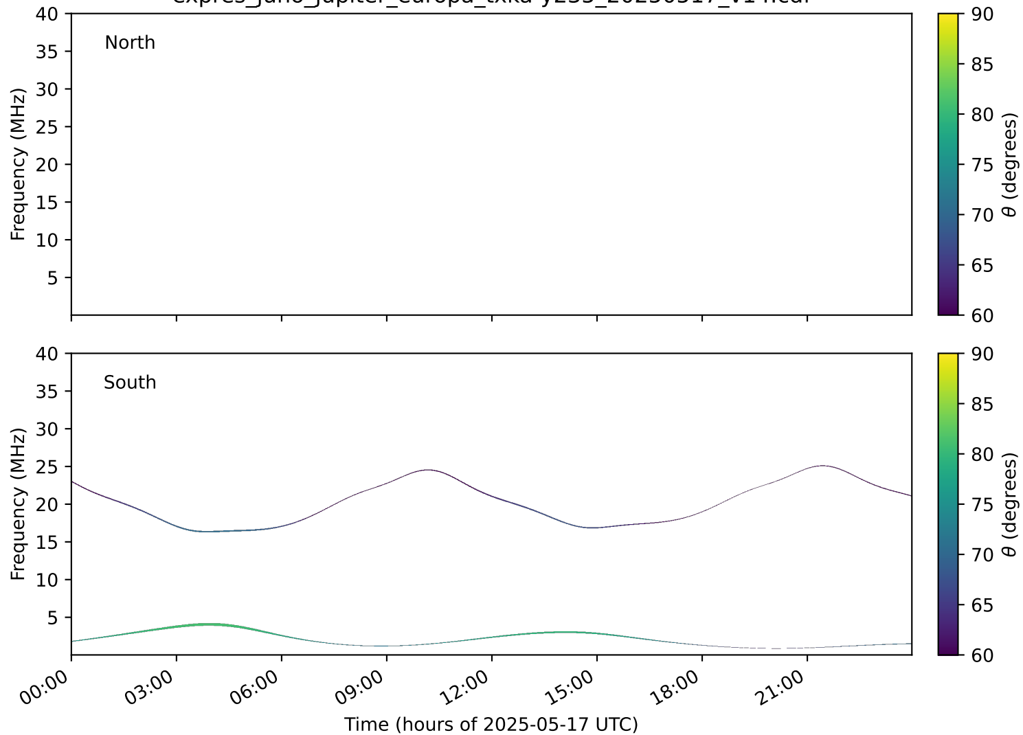
expres_juno_jupiter_europa_txka-y235_20250517_v14.cdf
