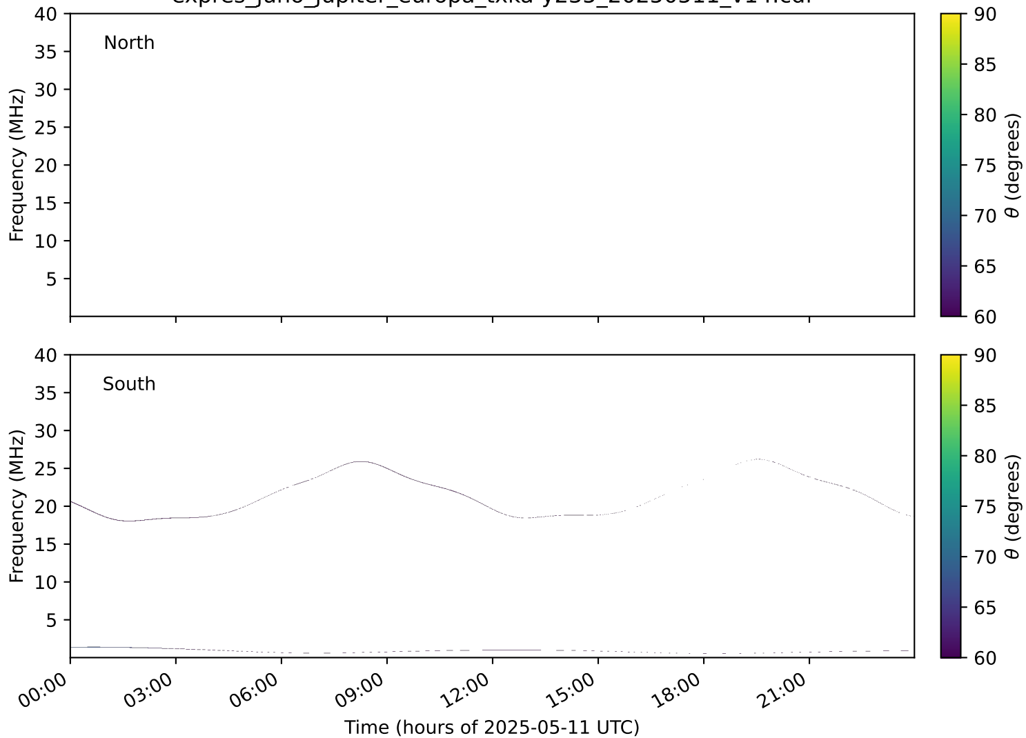
expres_juno_jupiter_europa_txka-y235_20250511_v14.cdf
