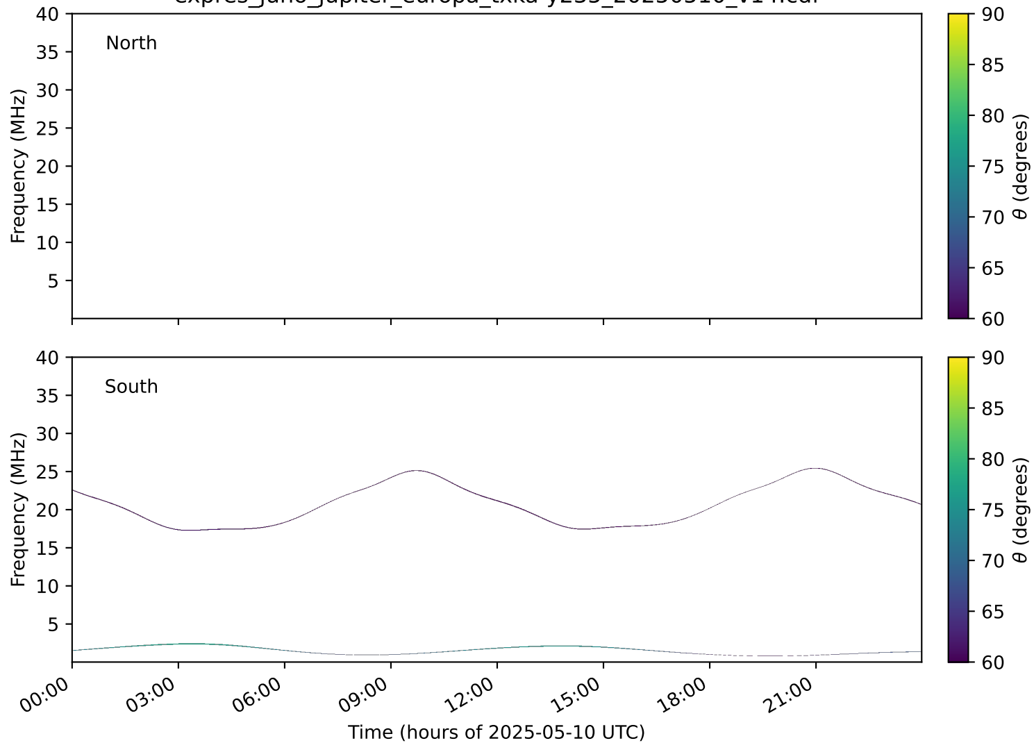
expres_juno_jupiter_europa_txka-y235_20250510_v14.cdf
