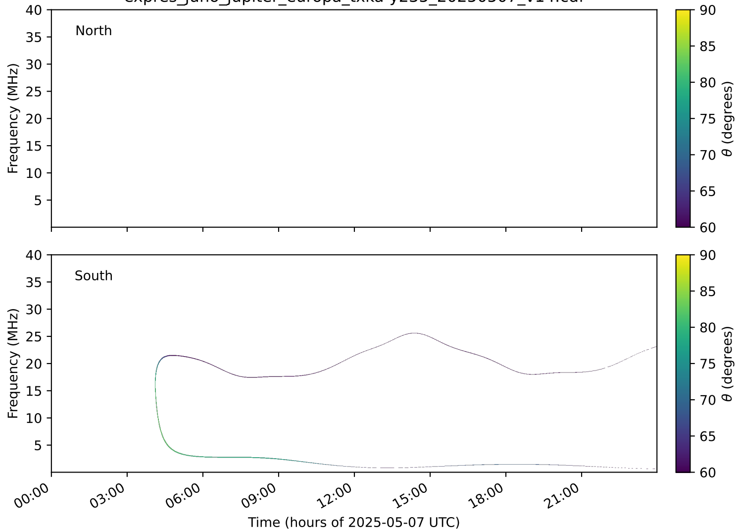
expres_juno_jupiter_europa_txka-y235_20250507_v14.cdf
