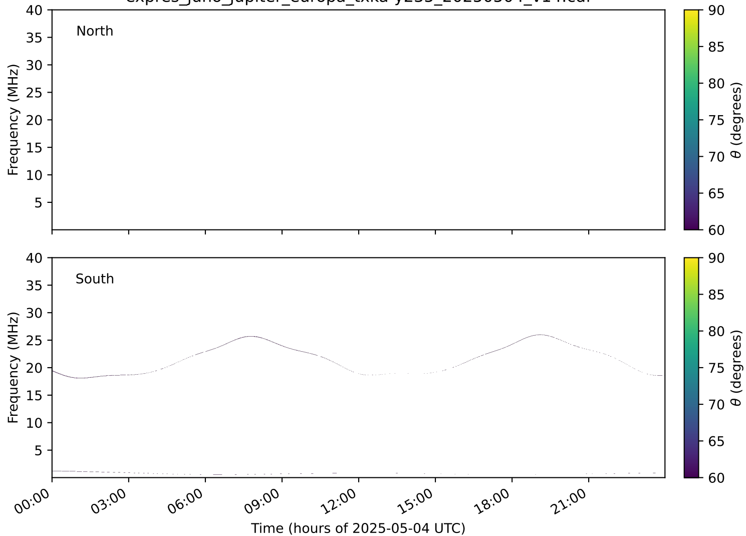
expres_juno_jupiter_europa_txka-y235_20250504_v14.cdf
