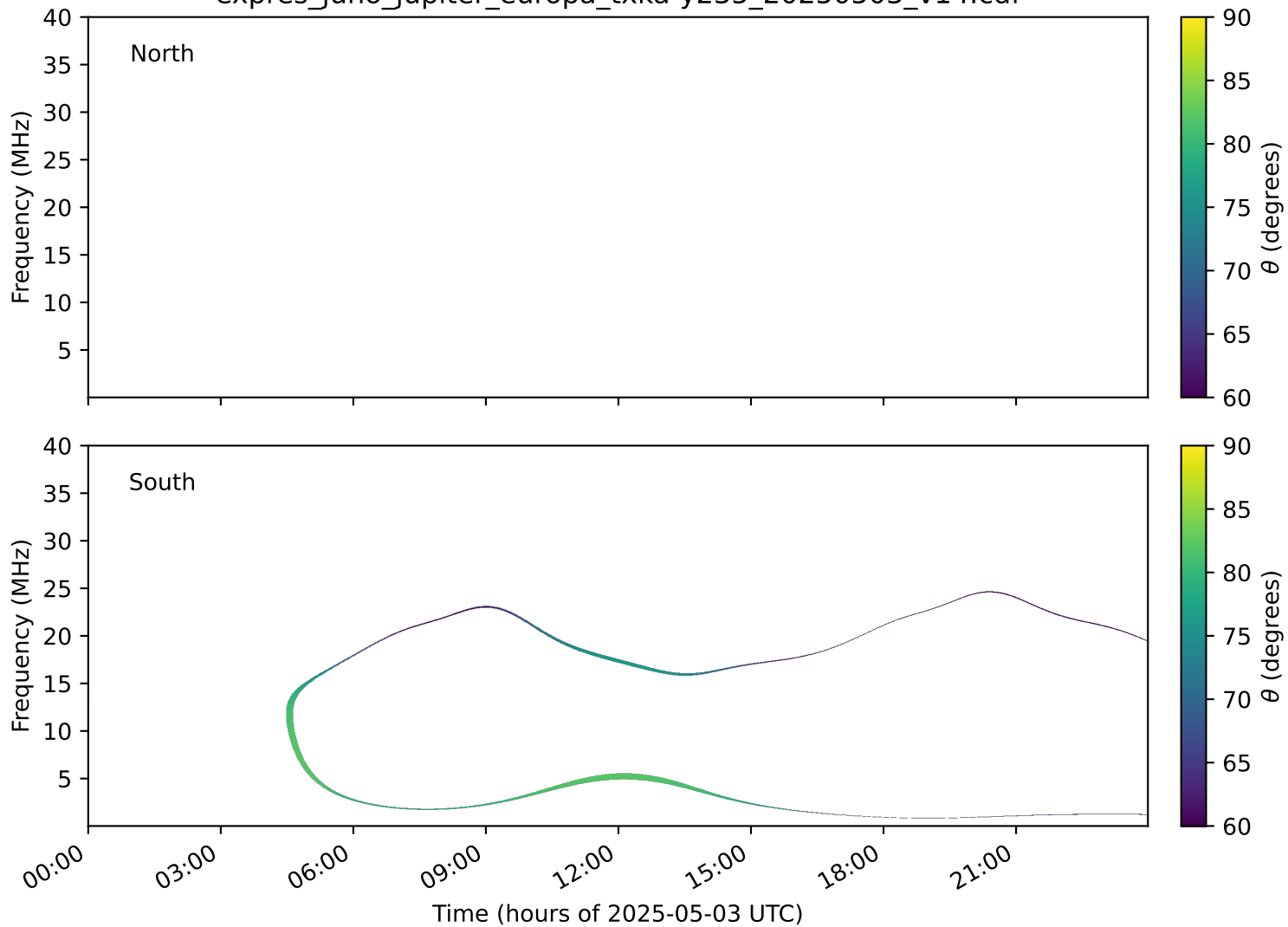
expres_juno_jupiter_europa_txka-y235_20250503_v14.cdf
