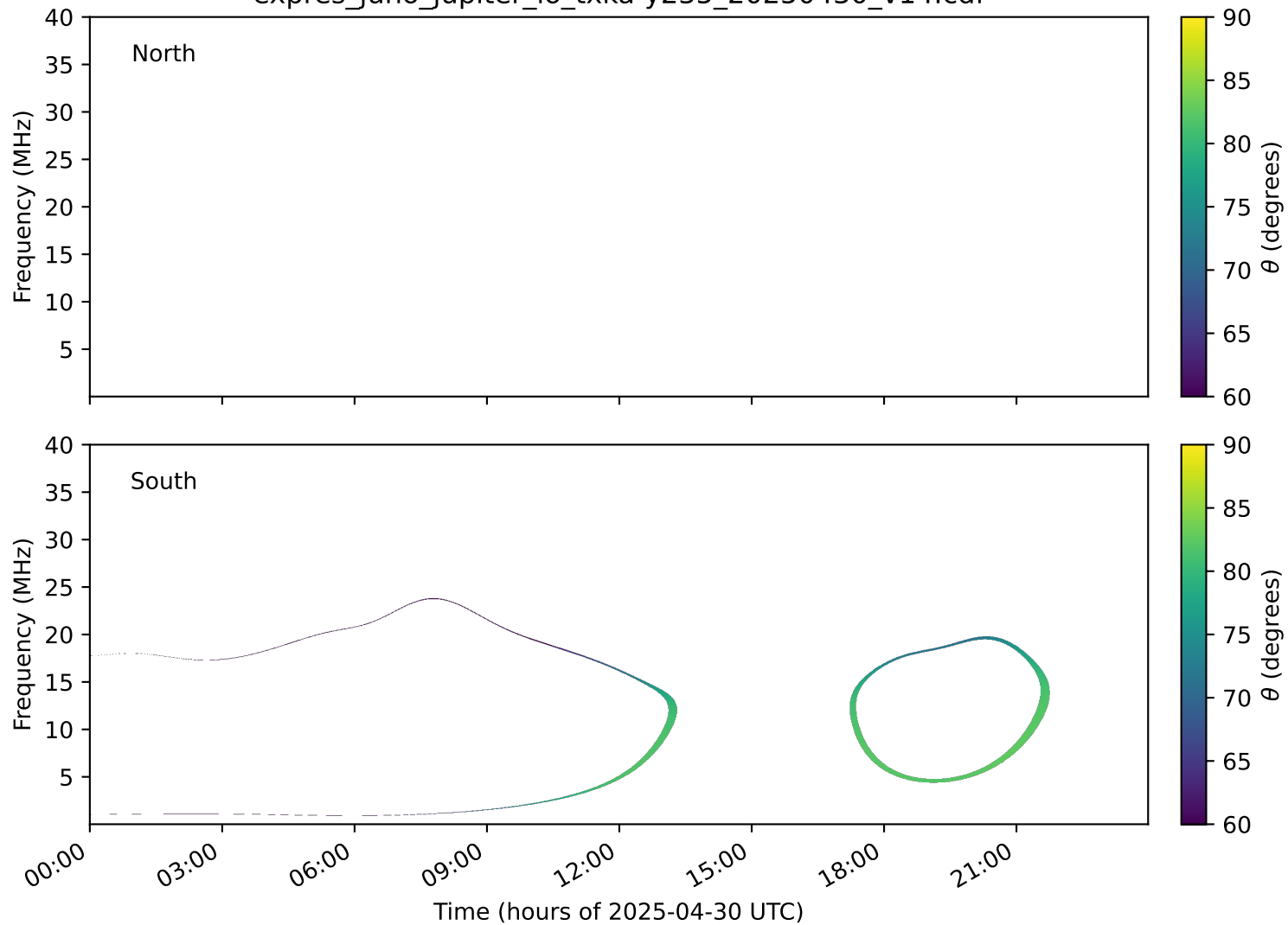
expres_juno_jupiter_io_txka-y235_20250430_v14.cdf
