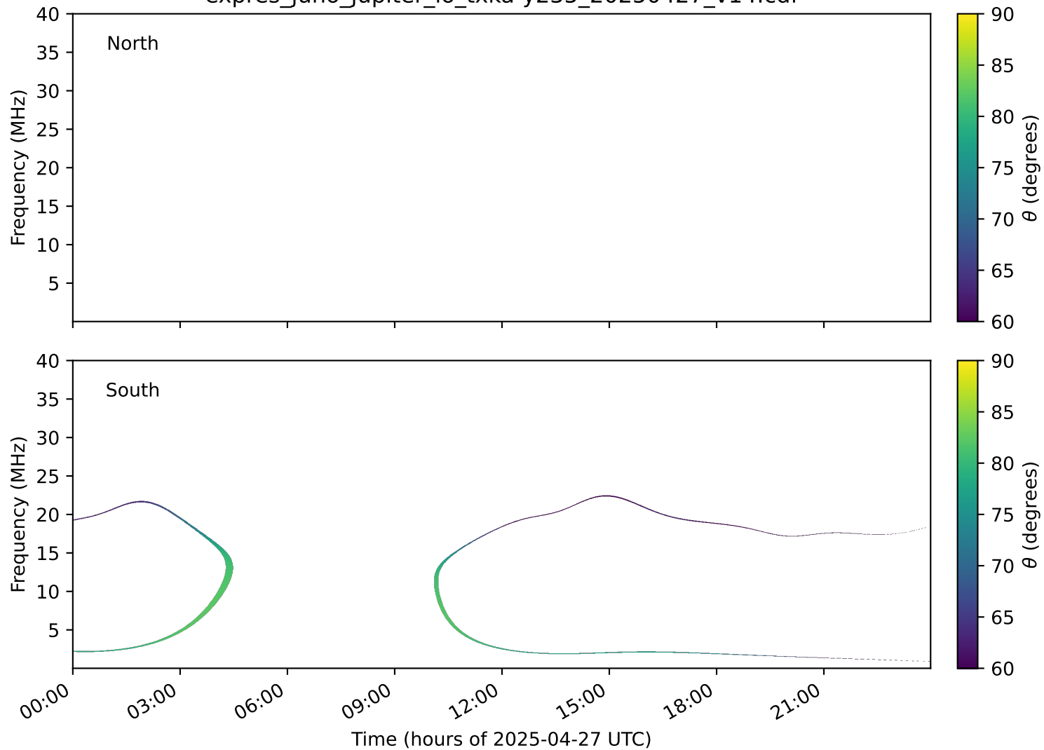
expres_juno_jupiter_io_txka-y235_20250427_v14.cdf
