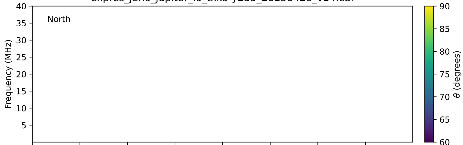
expres_juno_jupiter_io_txka-y235_20250426_v14.cdf
