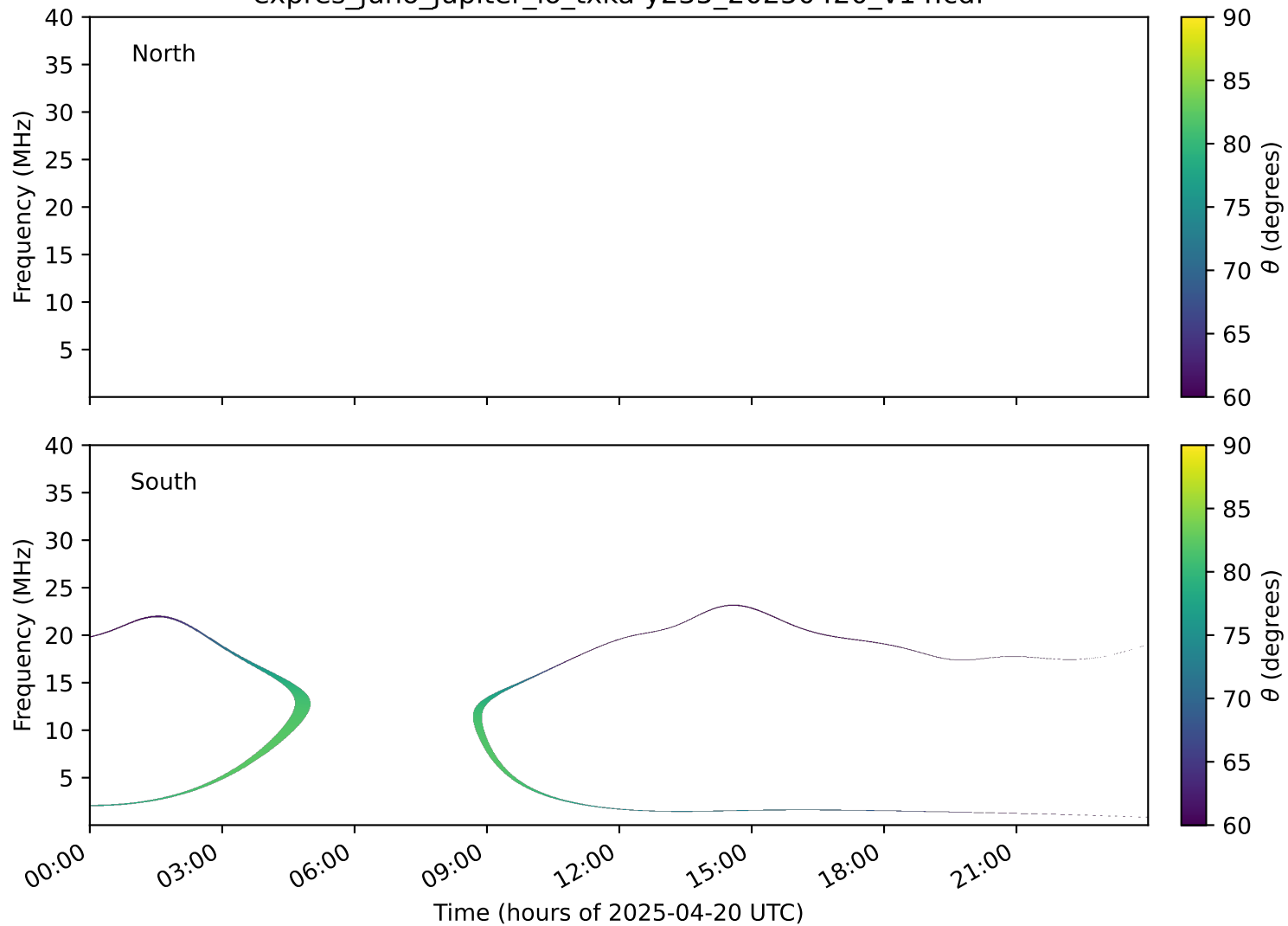
expres_juno_jupiter_io_txka-y235_20250420_v14.cdf
