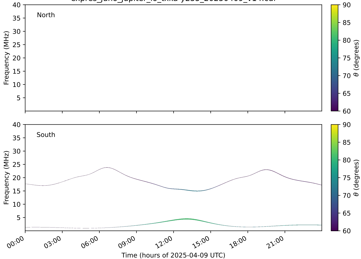
expres_juno_jupiter_io_txka-y235_20250409_v14.cdf
