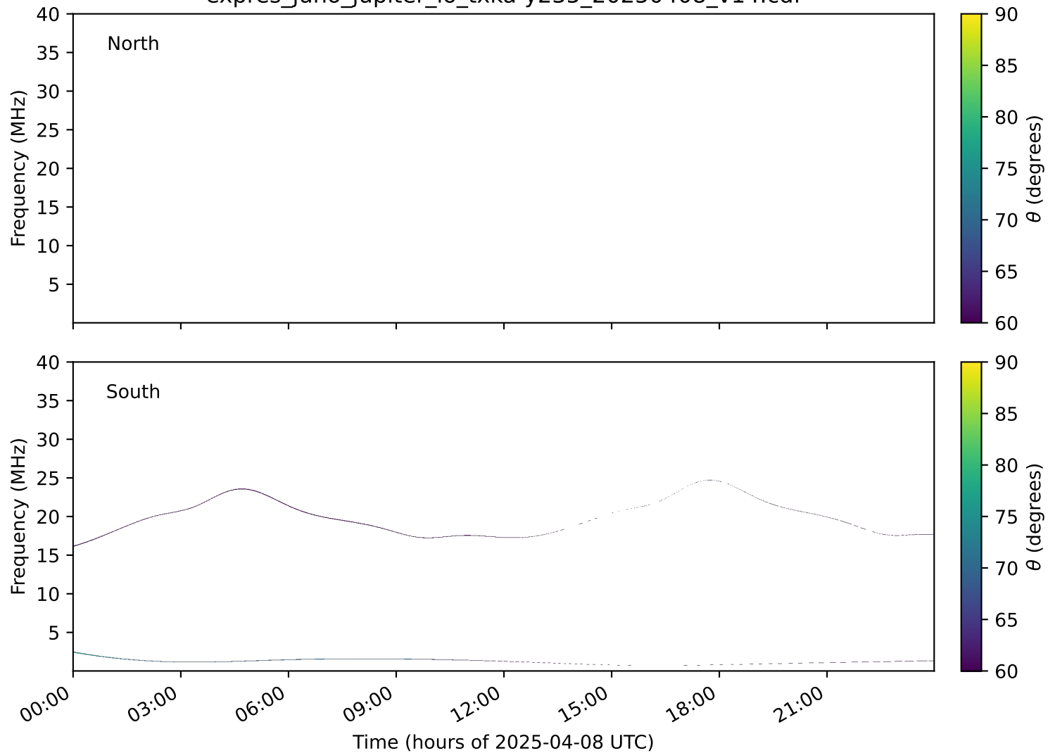
expres_juno_jupiter_io_txka-y235_20250408_v14.cdf
