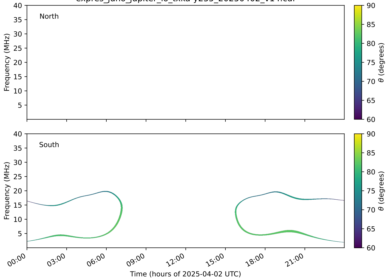
expres_juno_jupiter_io_txka-y235_20250402_v14.cdf
