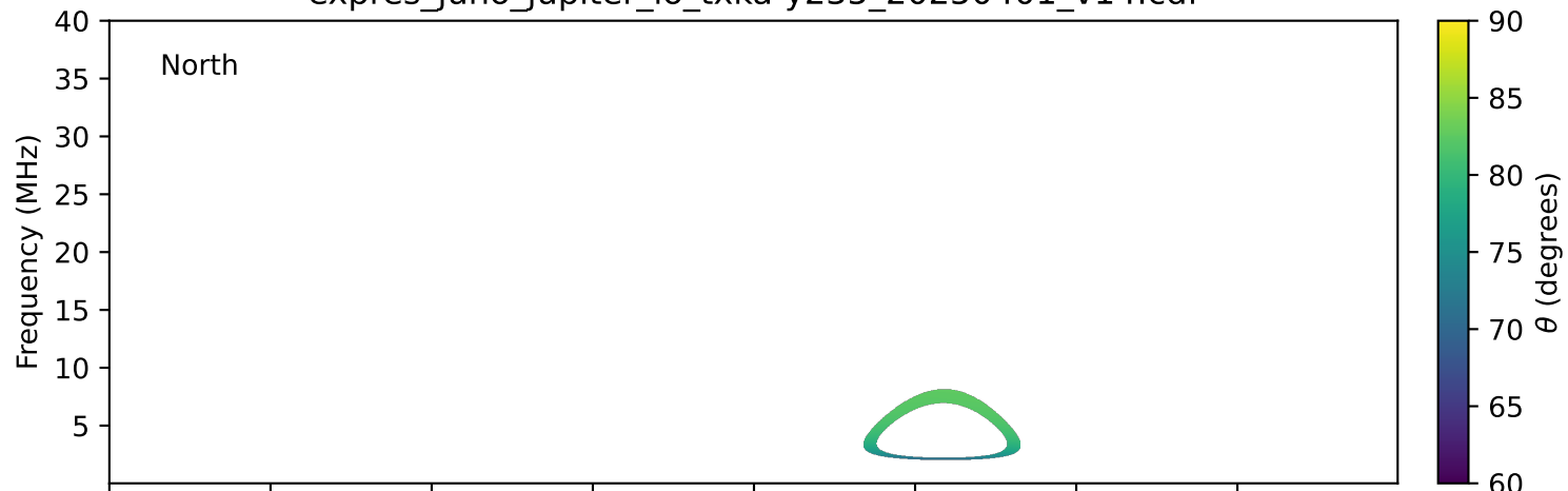
expres_juno_jupiter_io_txka-y235_20250401_v14.cdf
