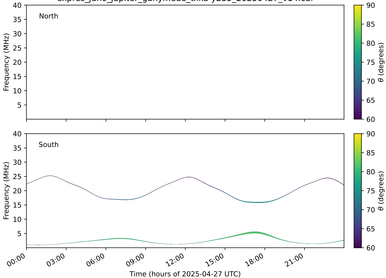
expres_juno_jupiter_ganymede_txka-y235_20250427_v14.cdf
