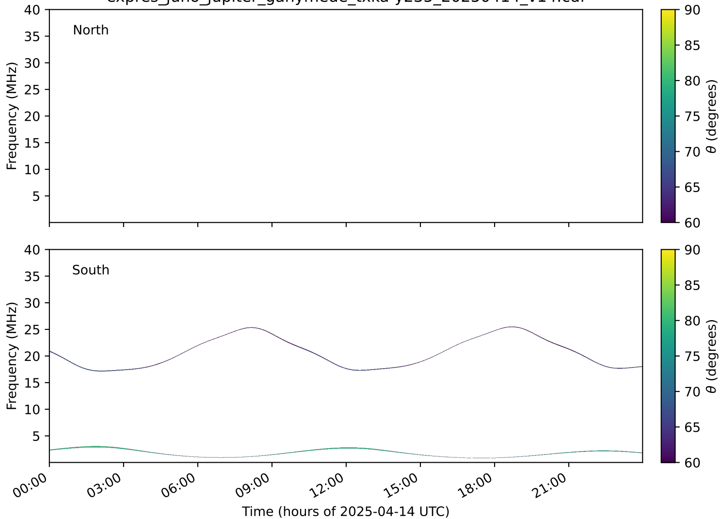
expres_juno_jupiter_ganymede_txka-y235_20250414_v14.cdf
