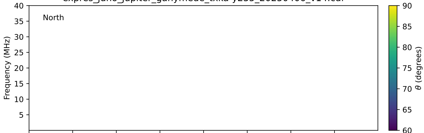
expres_juno_jupiter_ganymede_txka-y235_20250406_v14.cdf
