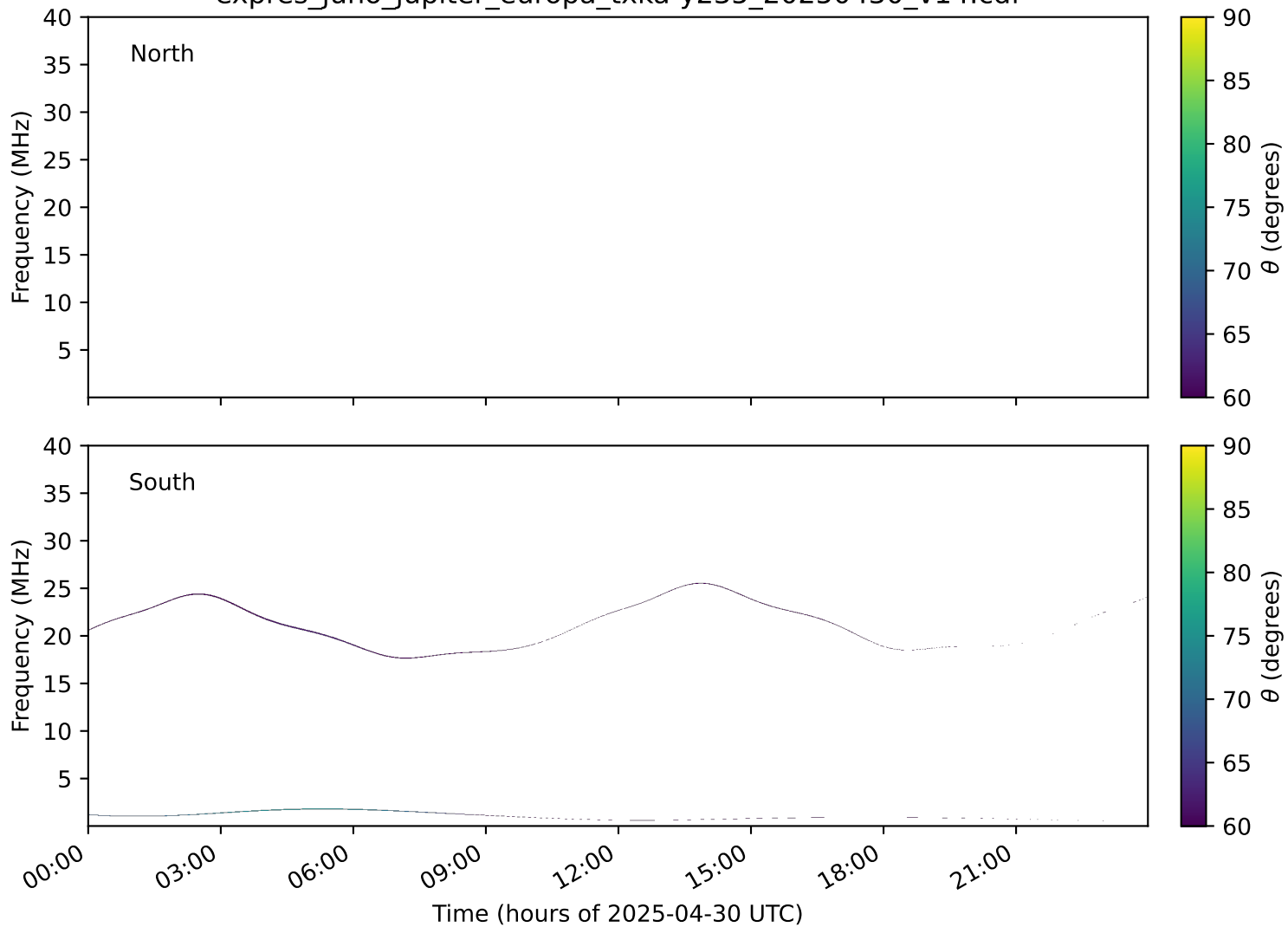
expres_juno_jupiter_europa_txka-y235_20250430_v14.cdf
