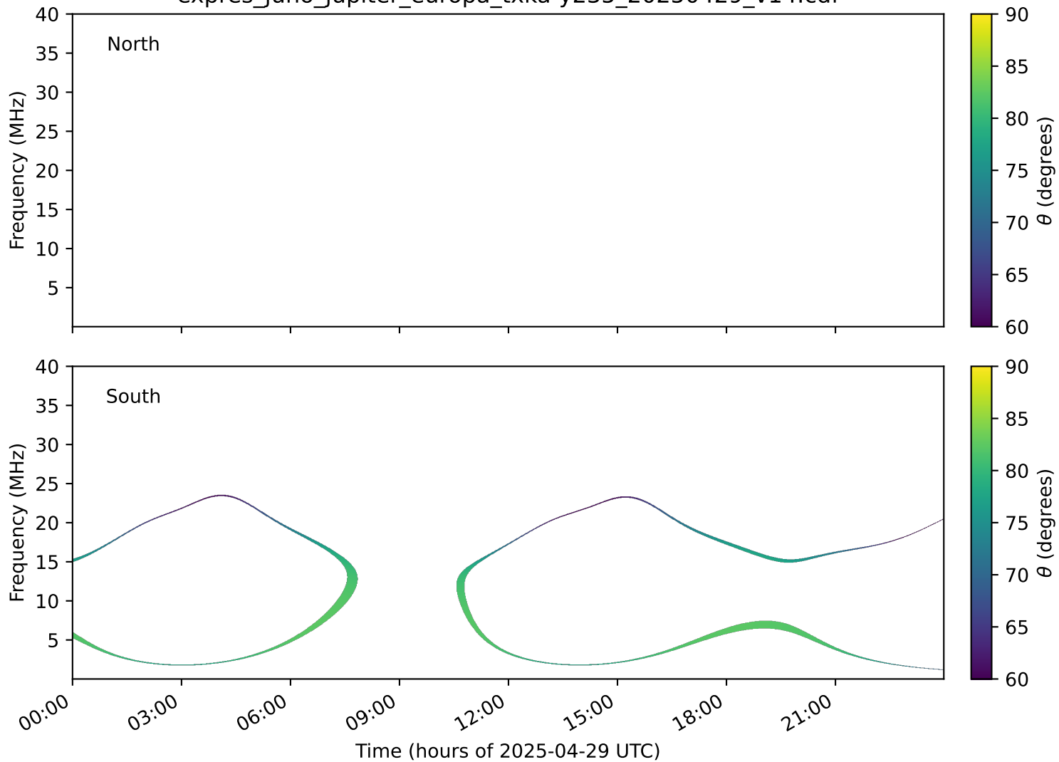
expres_juno_jupiter_europa_txka-y235_20250429_v14.cdf
