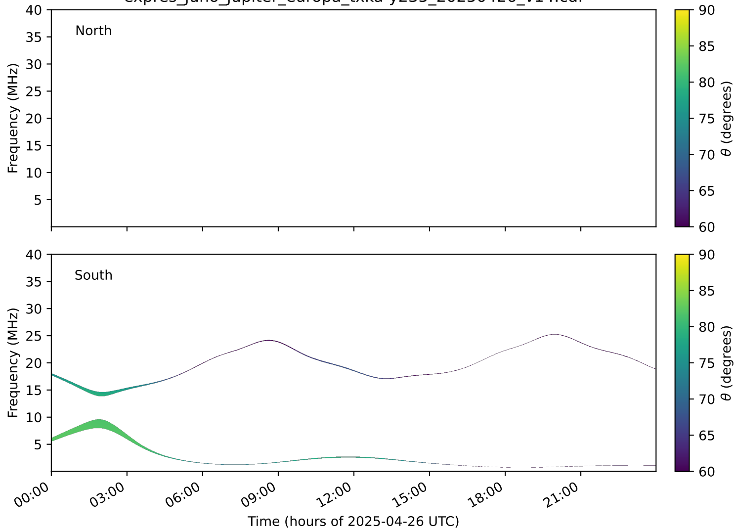
expres_juno_jupiter_europa_txka-y235_20250426_v14.cdf
