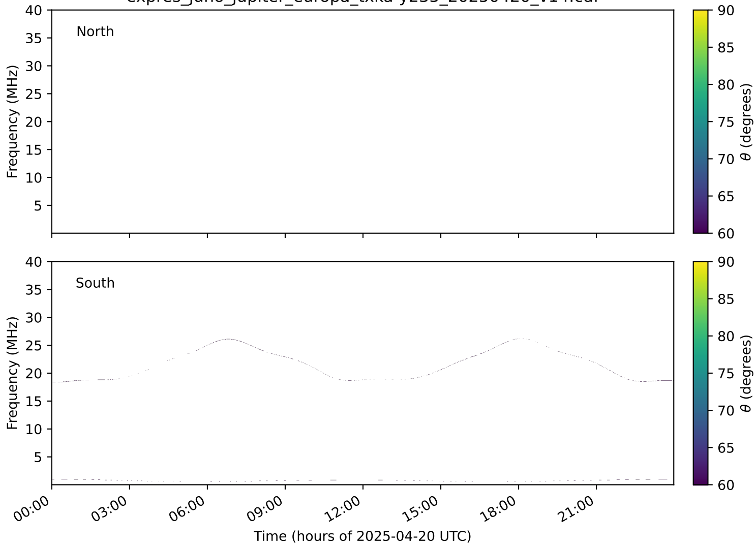
expres_juno_jupiter_europa_txka-y235_20250420_v14.cdf
