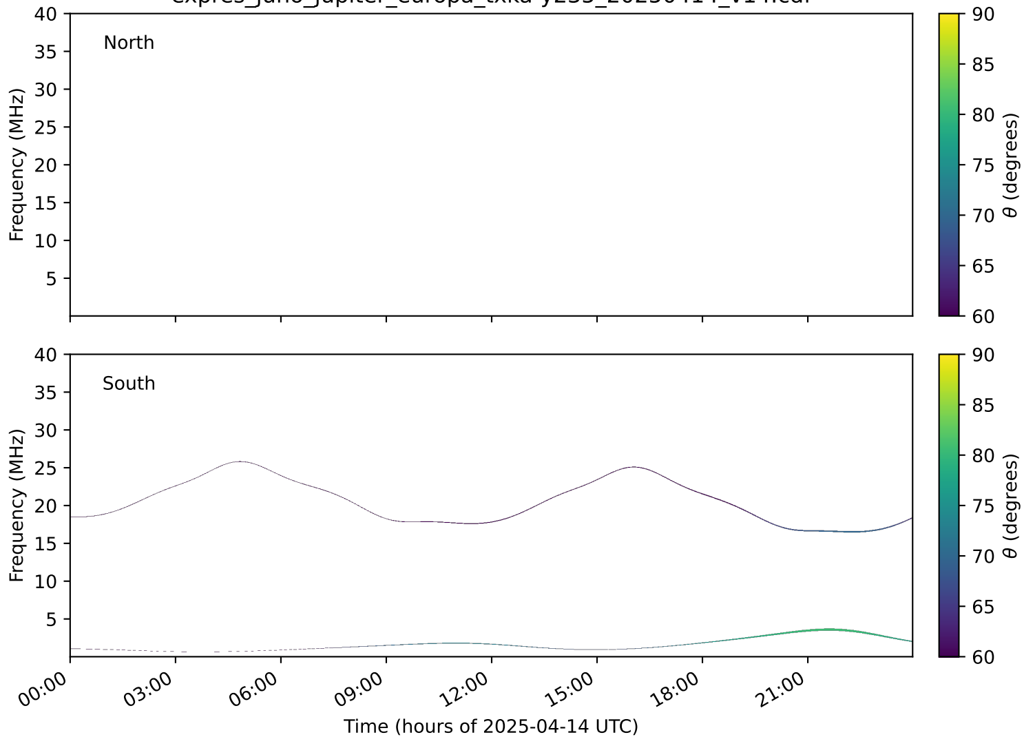
expres_juno_jupiter_europa_txka-y235_20250414_v14.cdf
