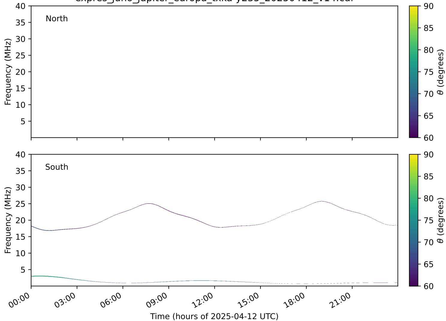
expres_juno_jupiter_europa_txka-y235_20250412_v14.cdf
