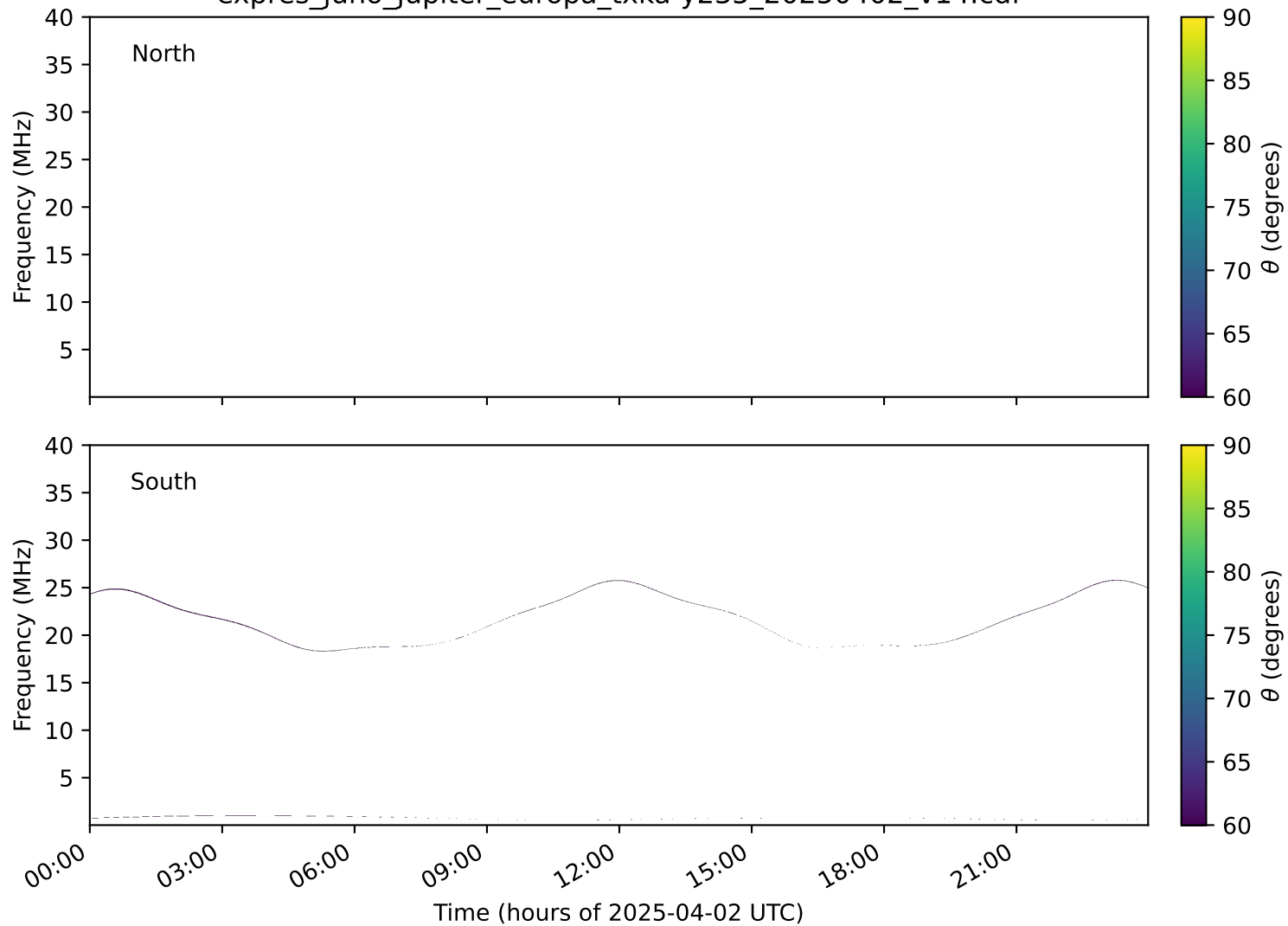
expres_juno_jupiter_europa_txka-y235_20250402_v14.cdf
