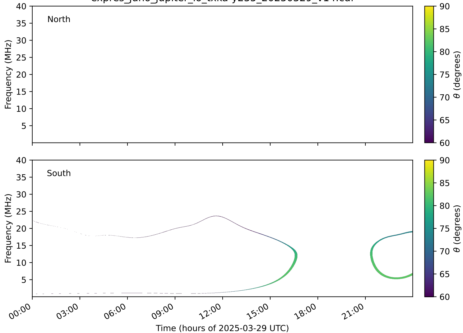
expres_juno_jupiter_io_txka-y235_20250329_v14.cdf
