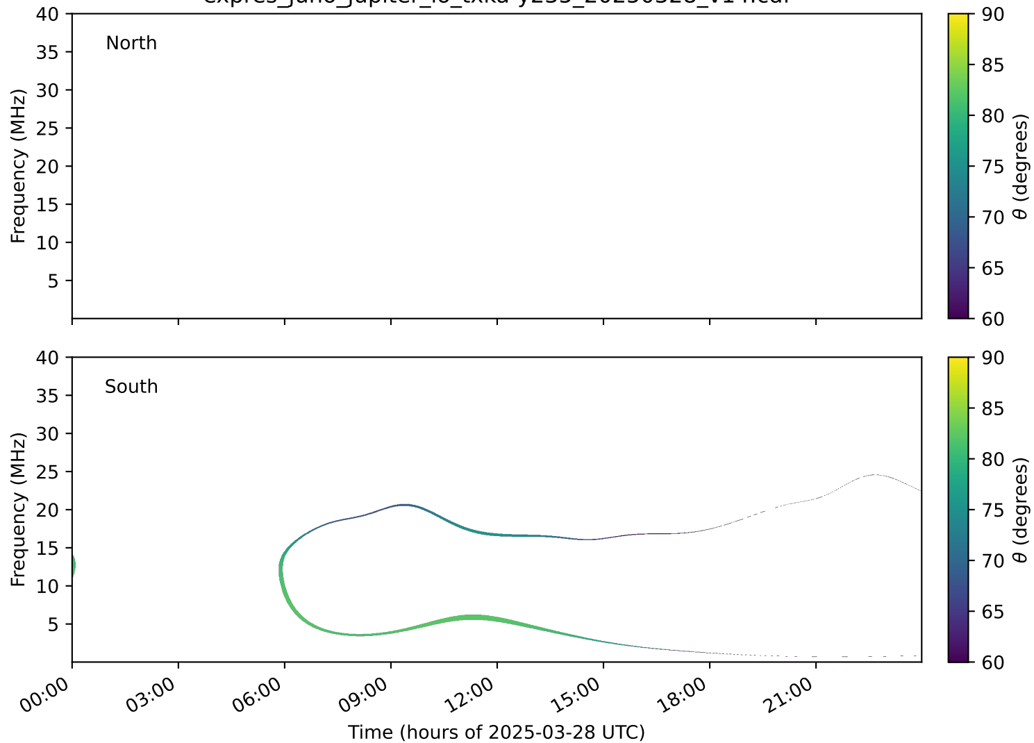
expres_juno_jupiter_io_txka-y235_20250328_v14.cdf
