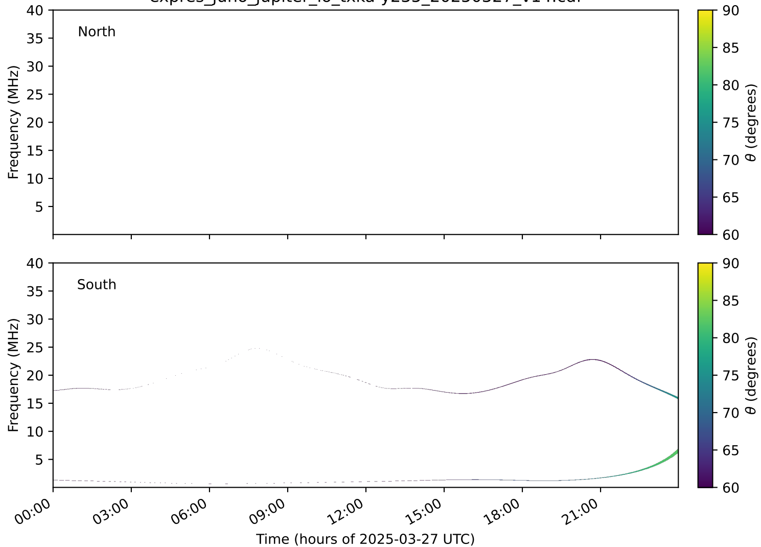
expres_juno_jupiter_io_txka-y235_20250327_v14.cdf
