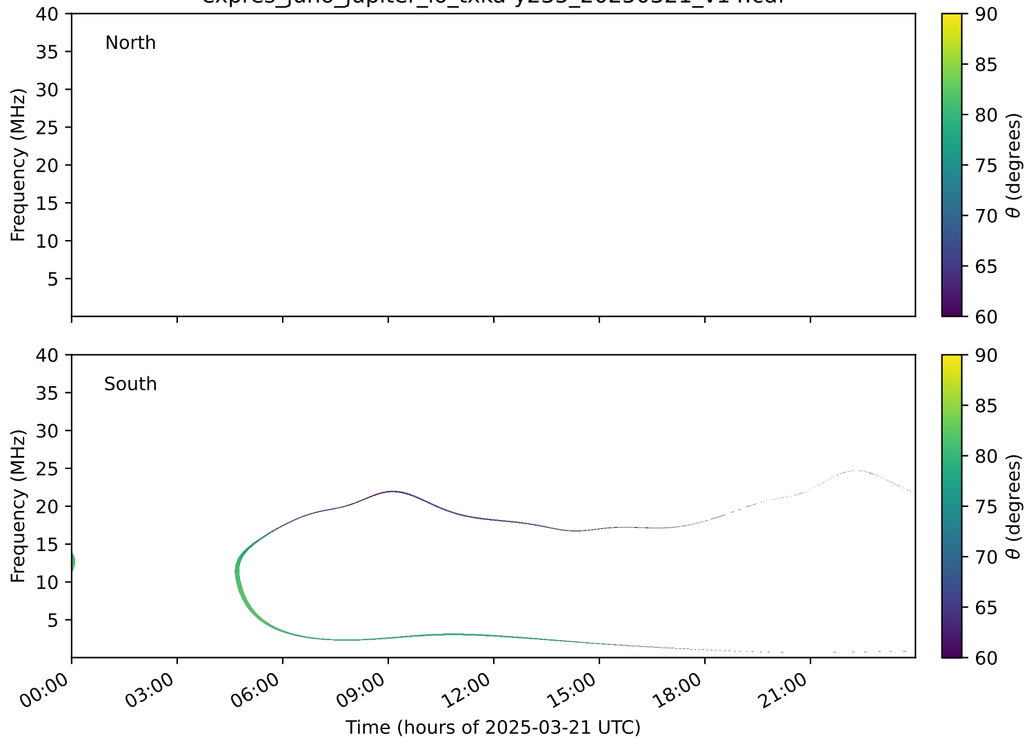
expres_juno_jupiter_io_txka-y235_20250321_v14.cdf
