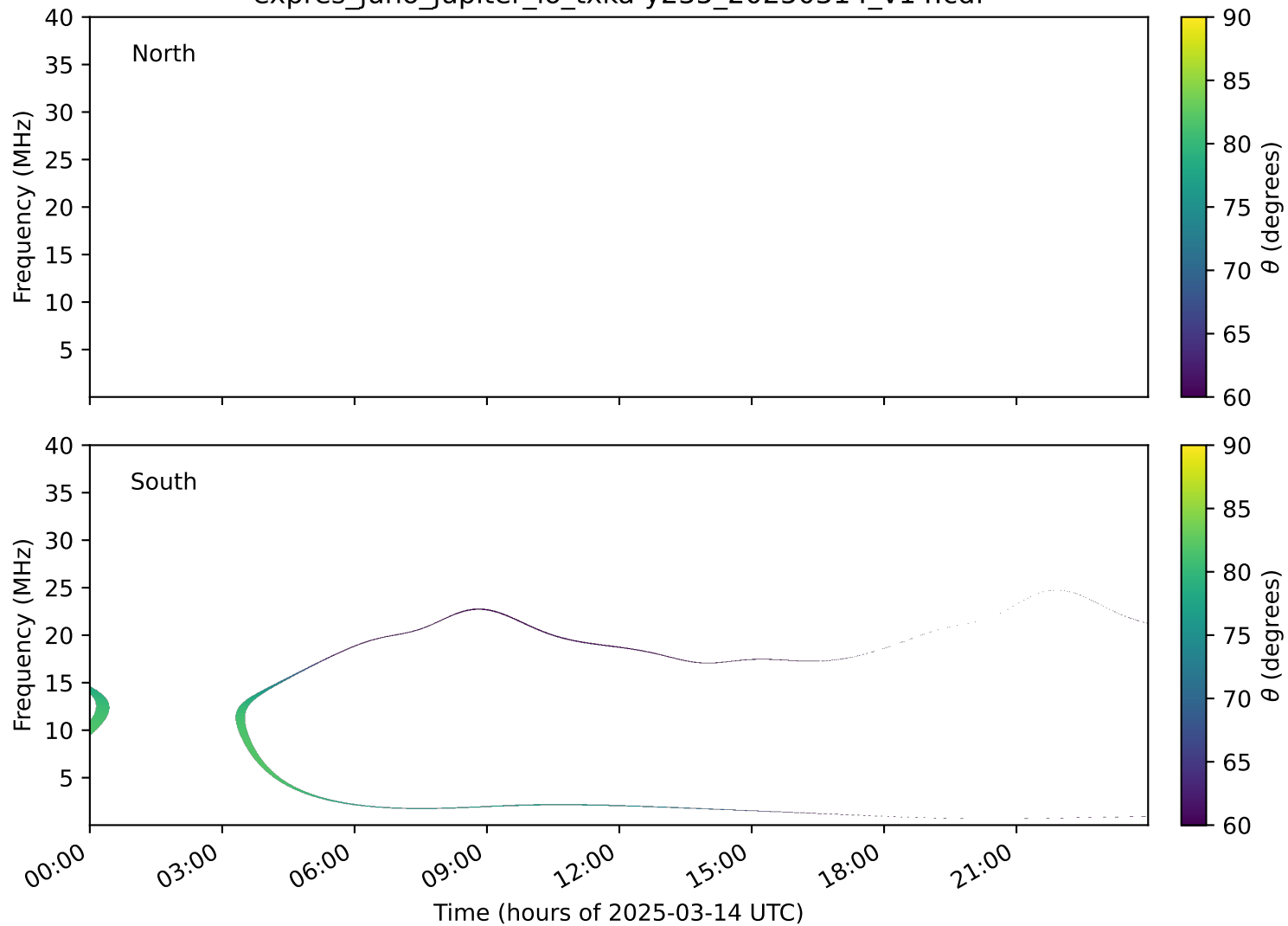
expres_juno_jupiter_io_txka-y235_20250314_v14.cdf
