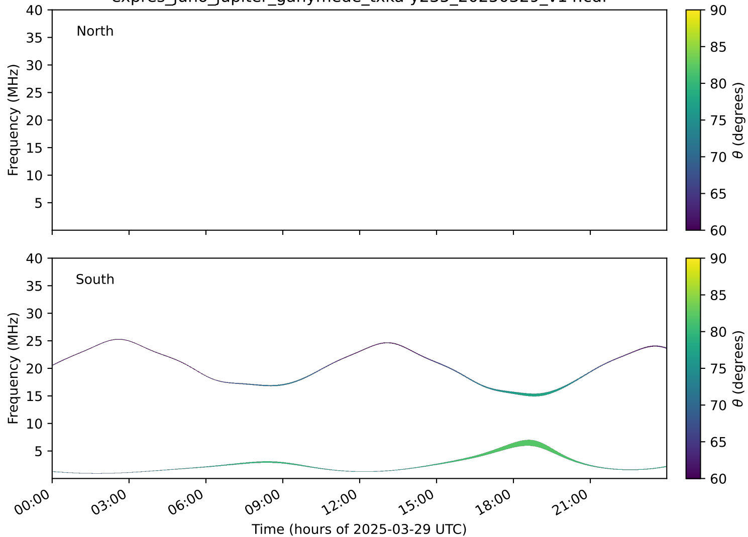
expres_juno_jupiter_ganymede_txka-y235_20250329_v14.cdf
