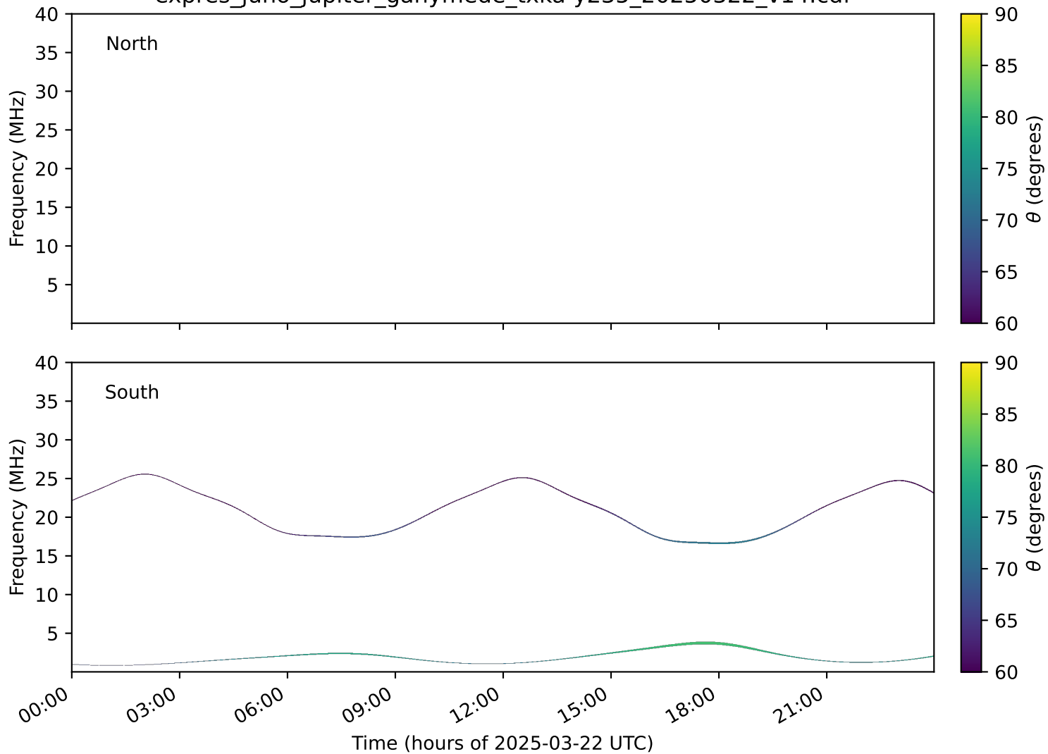
expres_juno_jupiter_ganymede_txka-y235_20250322_v14.cdf
