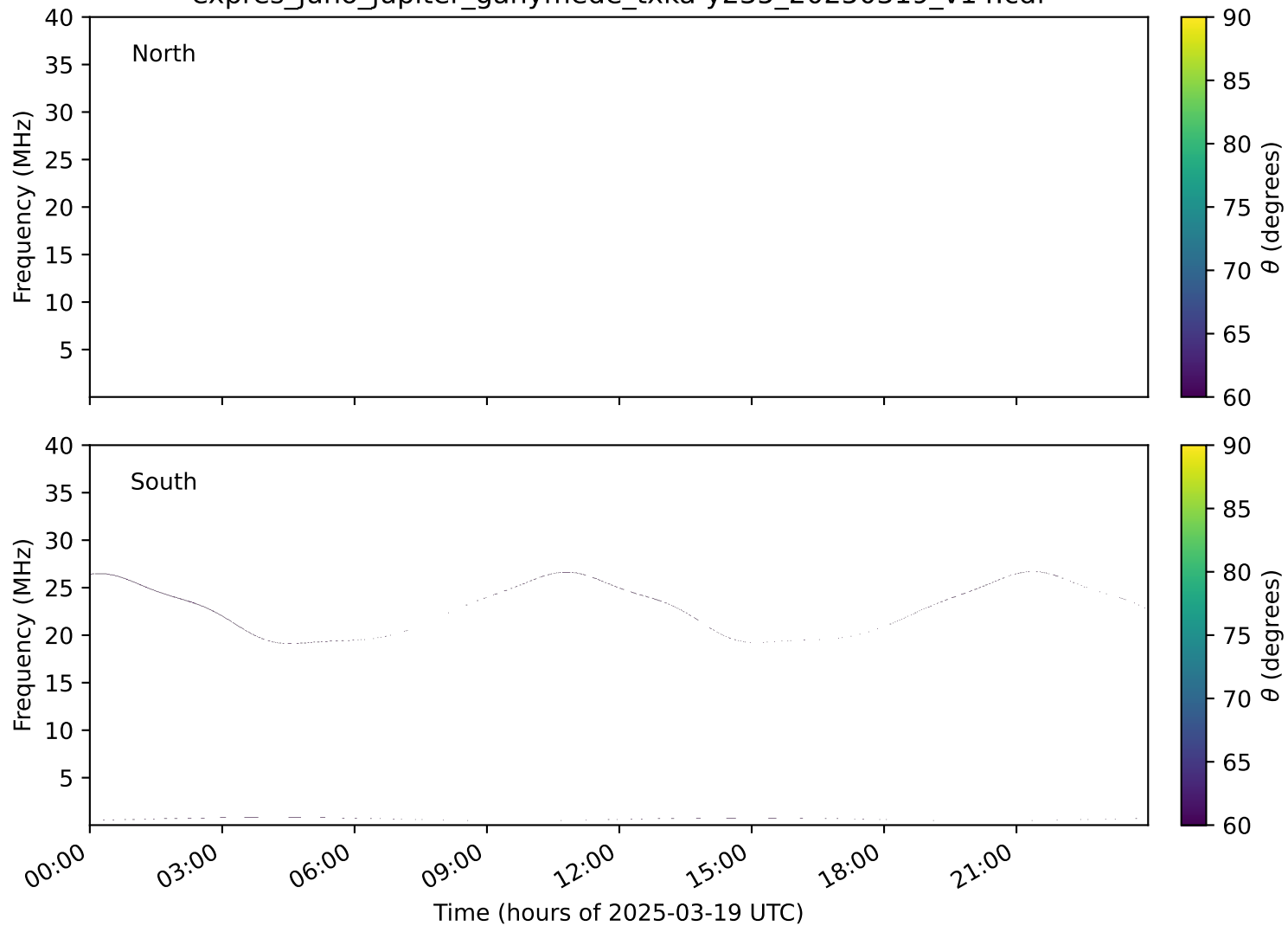
expres_juno_jupiter_ganymede_txka-y235_20250319_v14.cdf
