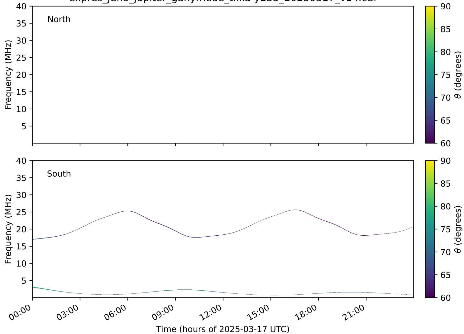
expres_juno_jupiter_ganymede_txka-y235_20250317_v14.cdf
