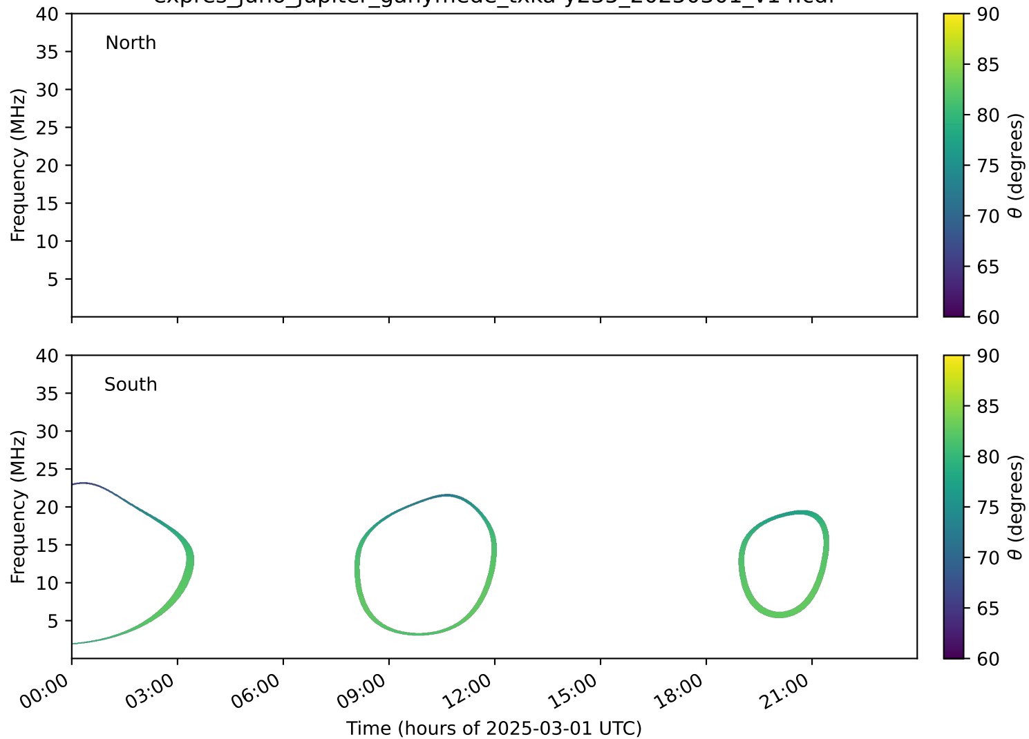
expres_juno_jupiter_ganymede_txka-y235_20250301_v14.cdf
