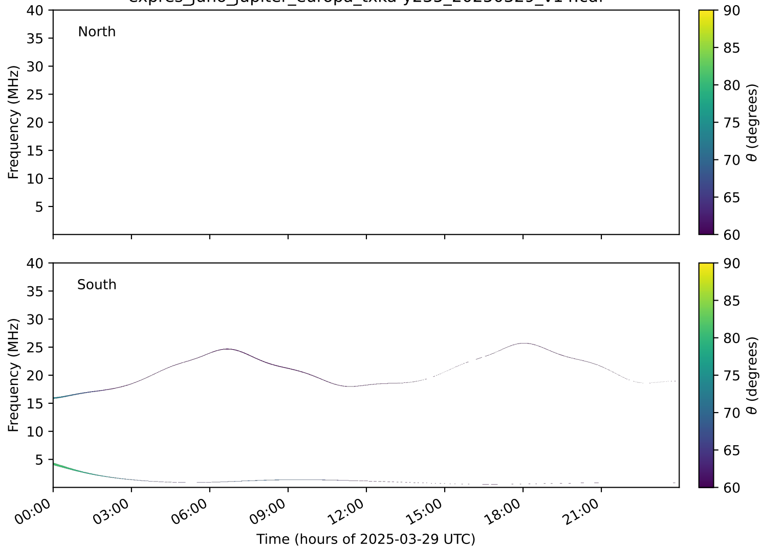
expres_juno_jupiter_europa_txka-y235_20250329_v14.cdf
