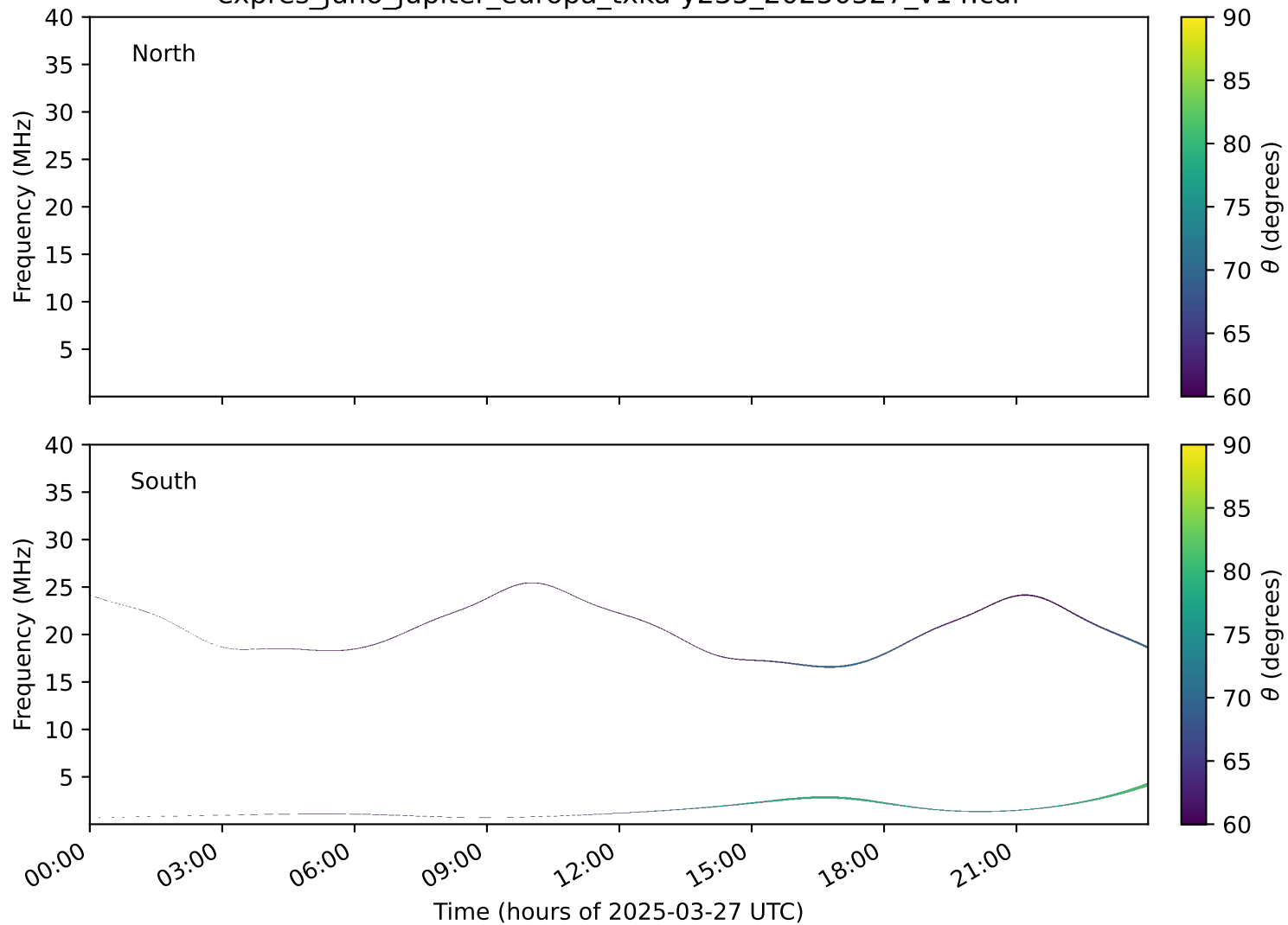
expres_juno_jupiter_europa_txka-y235_20250327_v14.cdf
