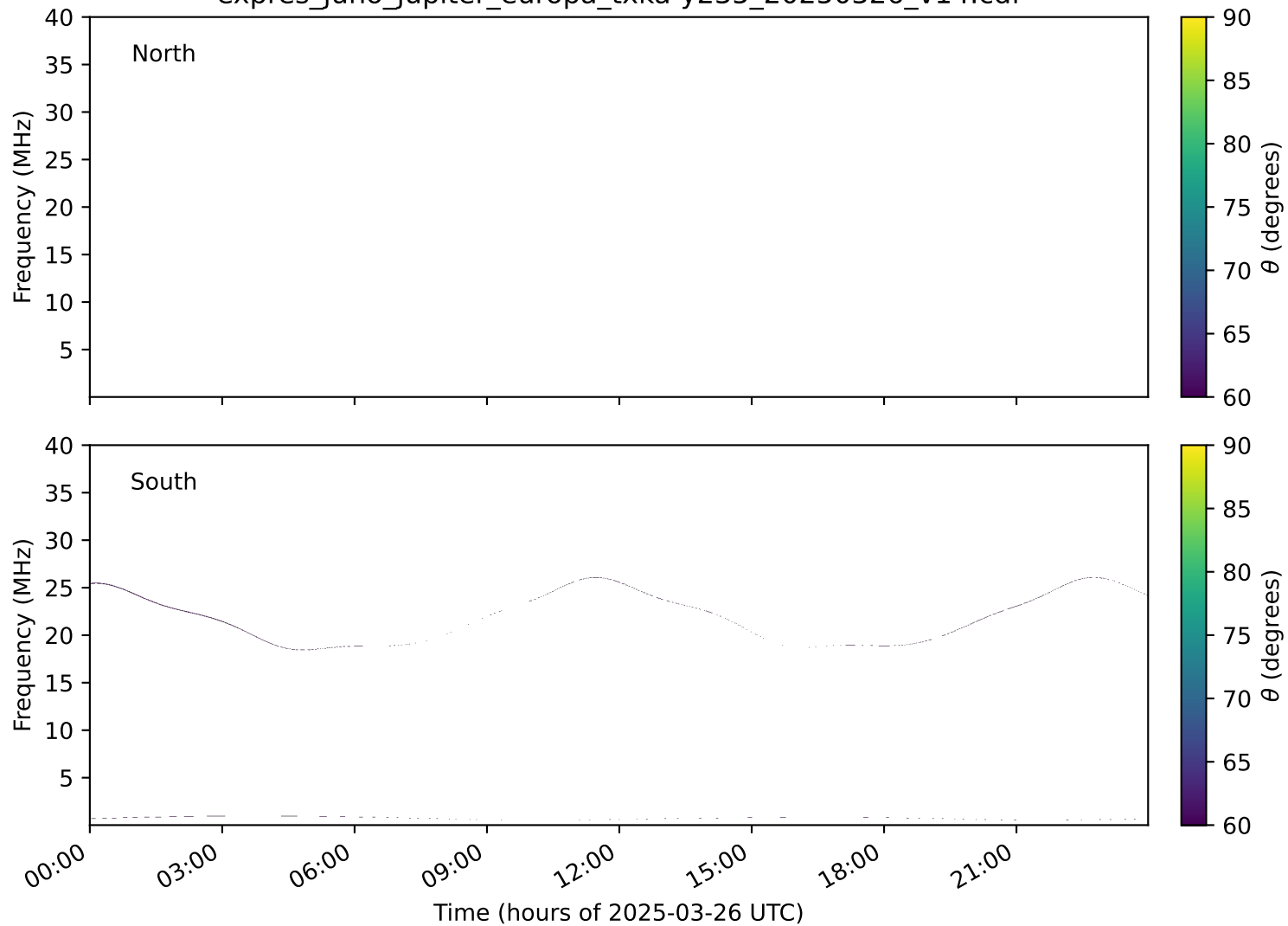
expres_juno_jupiter_europa_txka-y235_20250326_v14.cdf
