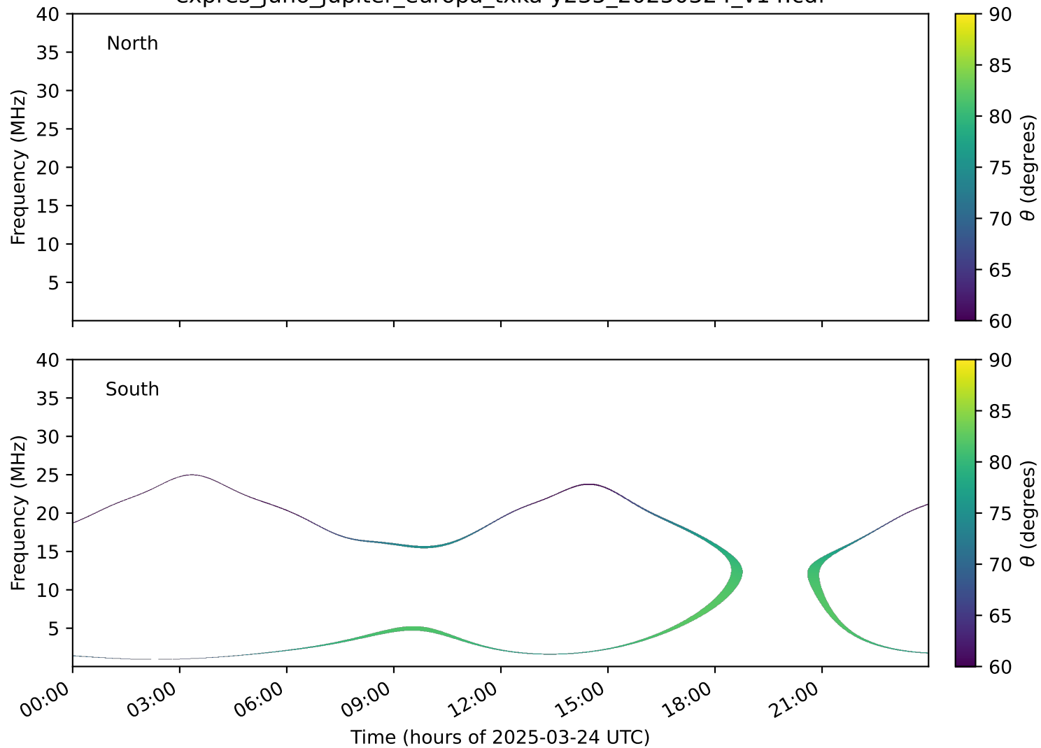
expres_juno_jupiter_europa_txka-y235_20250324_v14.cdf
