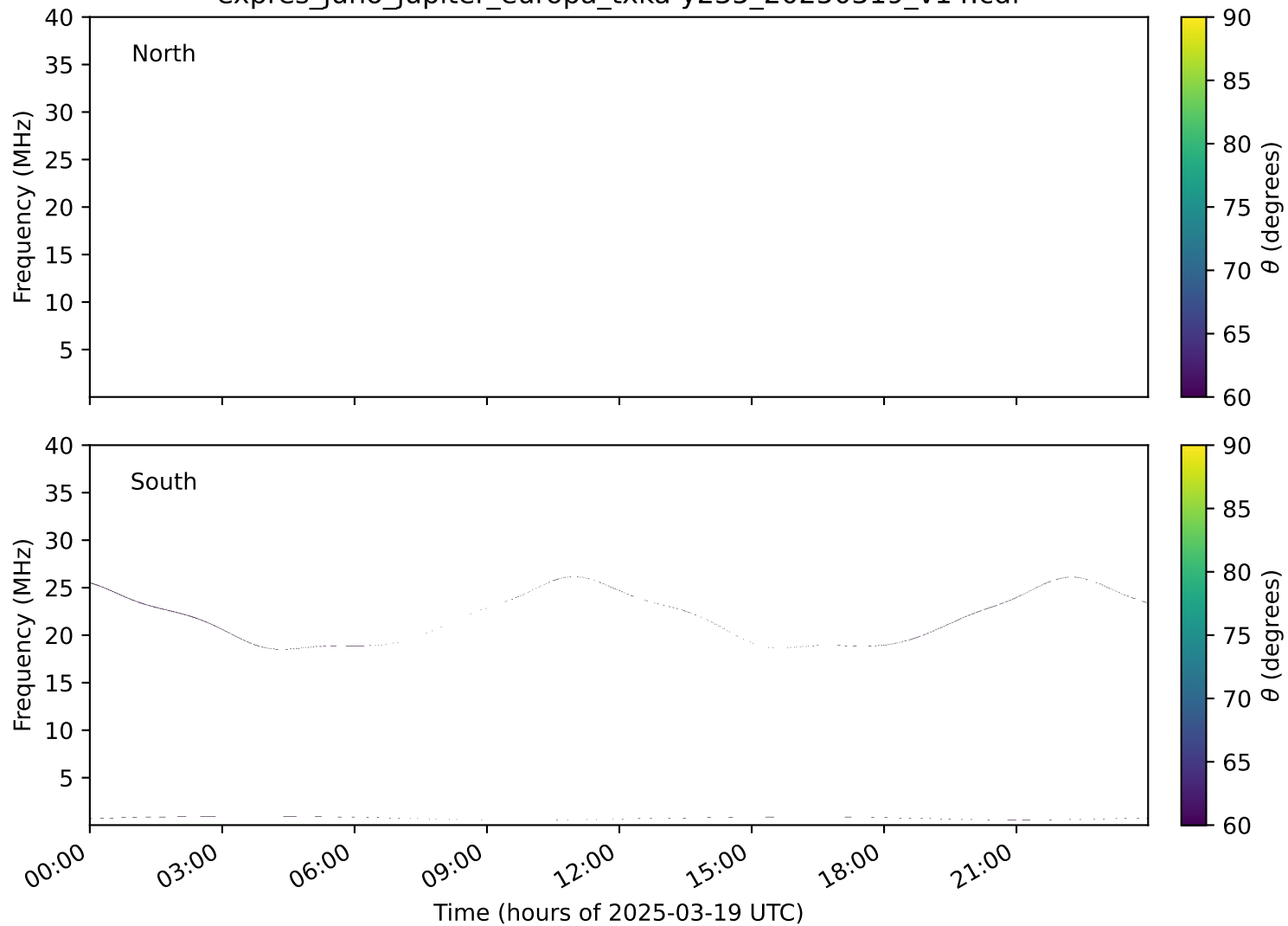
expres_juno_jupiter_europa_txka-y235_20250319_v14.cdf
