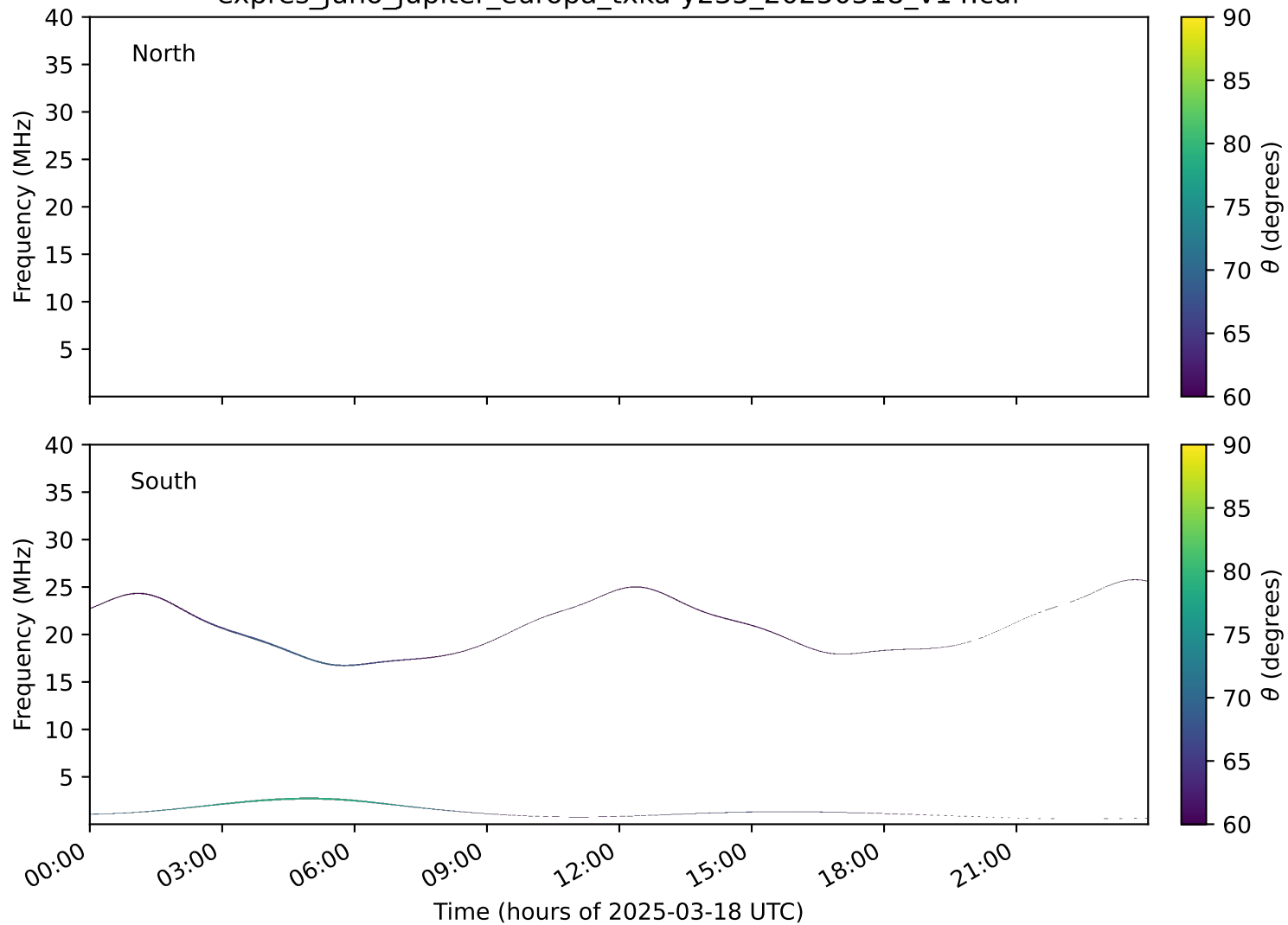
expres_juno_jupiter_europa_txka-y235_20250318_v14.cdf
